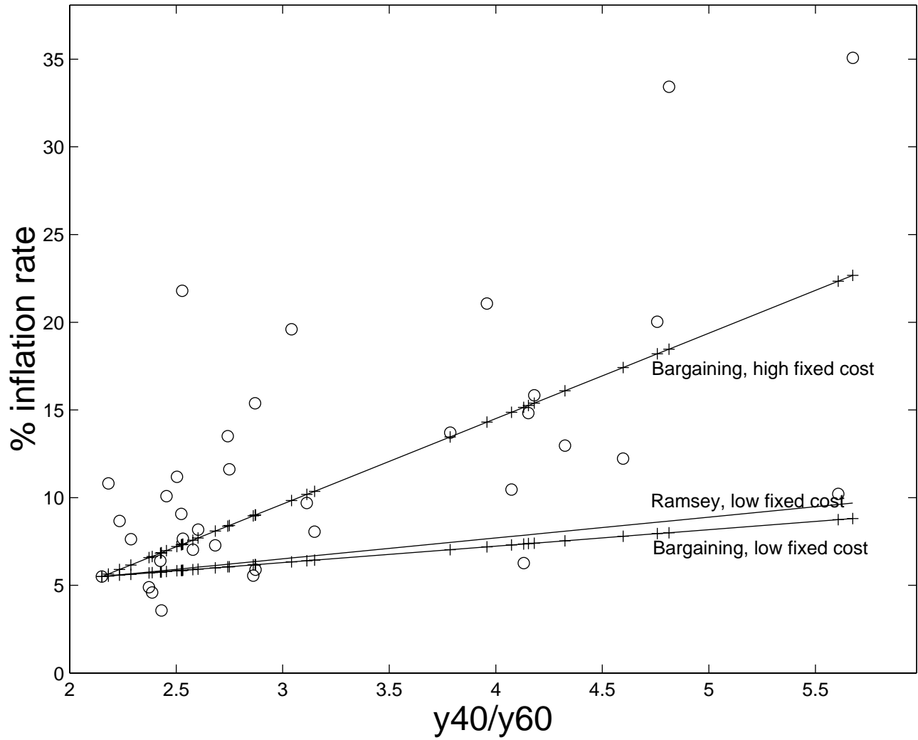
Figure 10: Predicted relation between inequality and inflation
