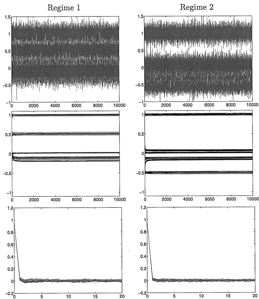
Figure C.2: Further results on convergence and efficiency
